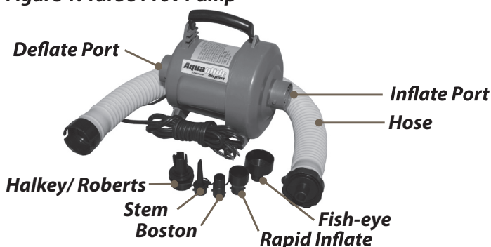
Figure 1: Turbo 110v Pump
