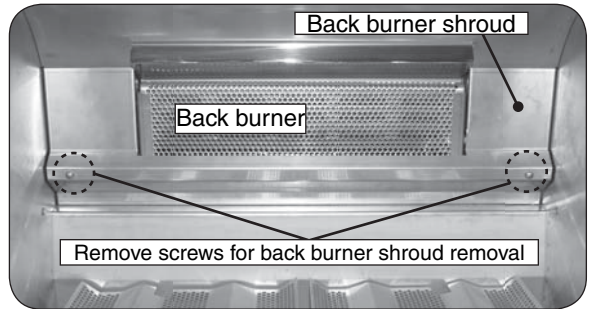
Fig. 1-1 Remove back burner shroud
