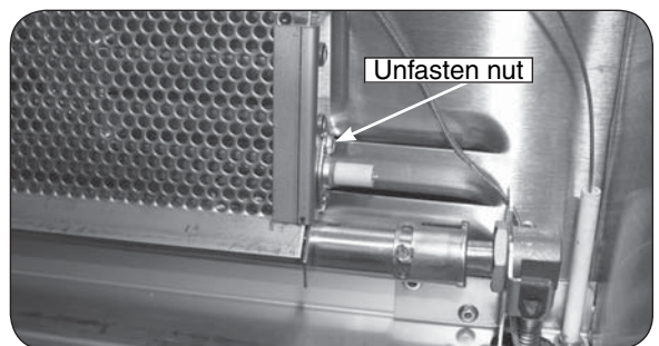
Fig. 1-3 Replace electrode
