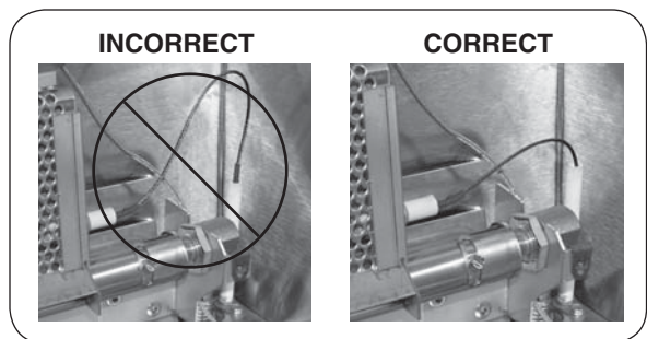
Fig. 1-4 New electrode wire placement
