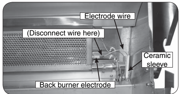
Fig. 1-2 Electrode & wire exposed
