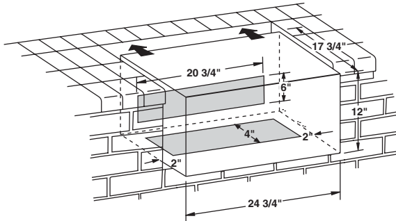
Figure 2 - Gas Stub Diagram
