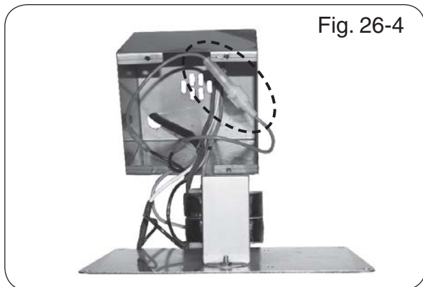
Carefully open box and replace fuse (red wire)
