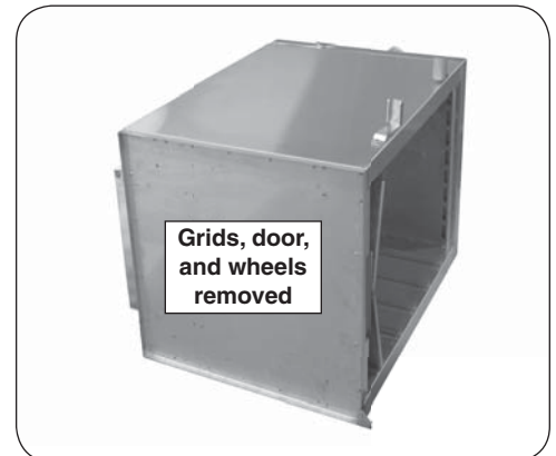
Fig. 1-1 Smoker on its side for base drawer install
