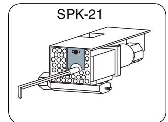
Fig. 5-3 ON position Burner on - Pilot on
